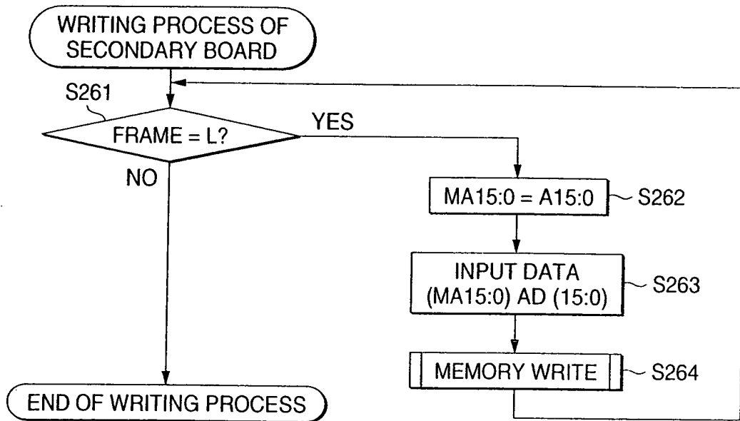
FIG. 24 PRIOR ART
